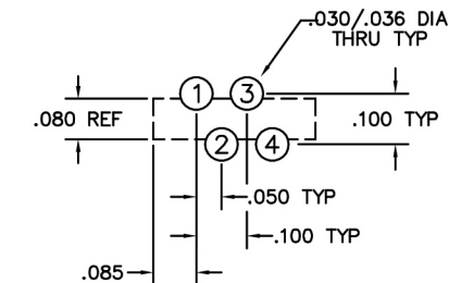
MATING FACE GUIDE HOLE (2 PLCS) PLUG MA-1H1-004-145-A6800
