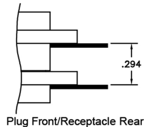
MOUNTING DIMENSIONS
