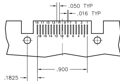
CONNECTOR MATING FACE
