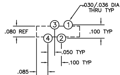
MATING FACE GUIDE PIN (2 PLCS) RECEPTACLE MA-1J1-004-245-A6700
