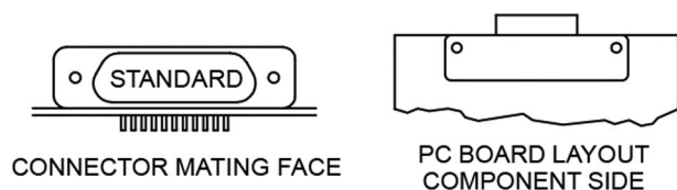
CONNECTOR MATING FACE (PLUG)
