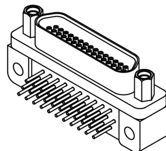
MK-2Q2-031-B45-220S (RECEPTACLE)
