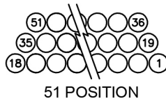
CONNECTOR MATING FACE (PLUG)
