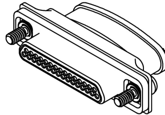
MM-2P2-031-113-4500 (PLUG)
