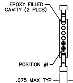
TERMINATION VIEW
