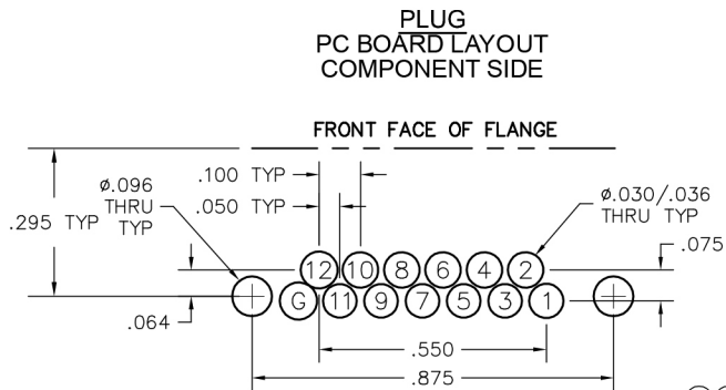
PC BOARD LAYOUT COMPONENT SIDE
