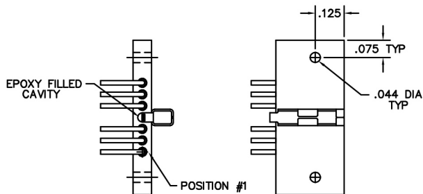
TERMINATION VIEW
