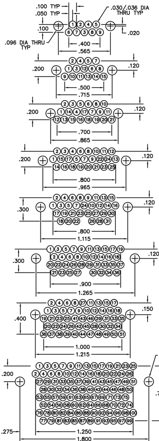
PLUG PC BOARD LAYOUT COMPONENT SIDE
