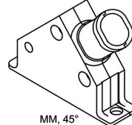
MM, 45° (TWO PIECE) (POSITIONS 21 - 100)
