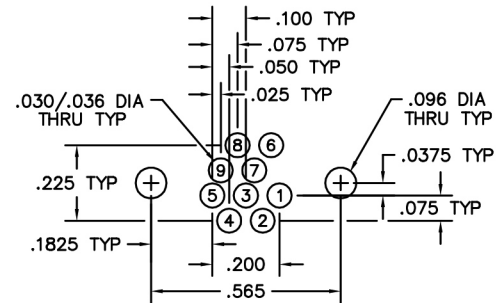
PLUG PC BOARD LAYOUT COMPONENT SIDE
