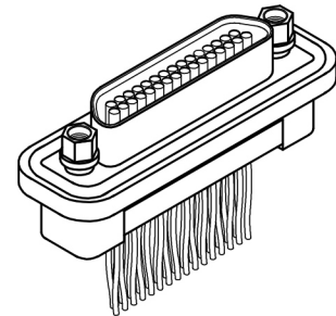
MM-2H2-031-261-26WA (RECEPTACLE)
