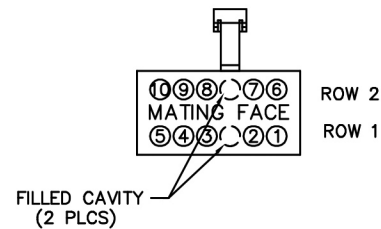
RECEPTACLE MA-241-010-261-ALCWA
