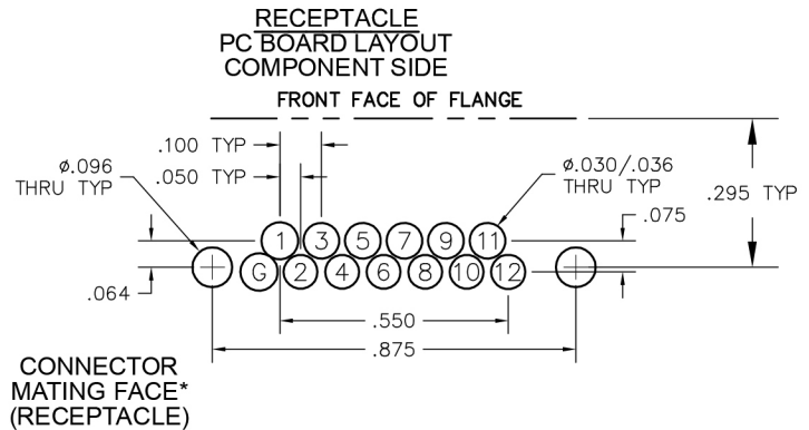
CONNECTOR MATING FACE* (RECEPTACLE) 12 POSITION
