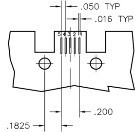
PLUG PC BOARD LAYOUT CIRCUIT SIDE
