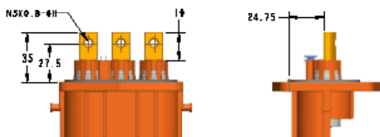
Busbar Type
