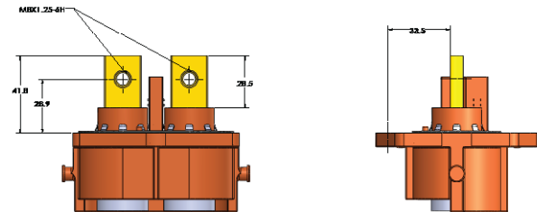
Busbar Type
