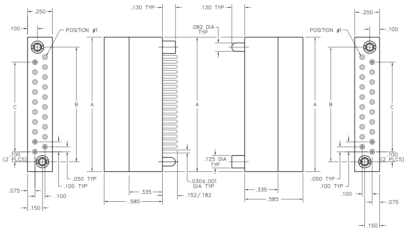
PLUG
