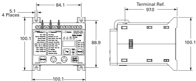
Mounting Dimension (4) 10-32
