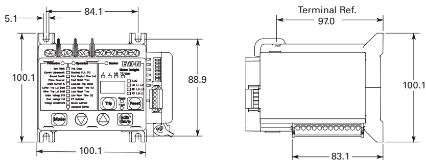
Mounting Dimensions (4) 10-32
