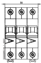
3-pole
